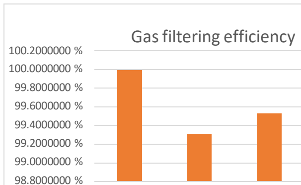
Figure 4. Gas (formaldehyde) filtering efficiency in Airforte Aero BMG purifier at different speeds.
